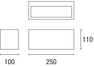
Uplight / Downlight
